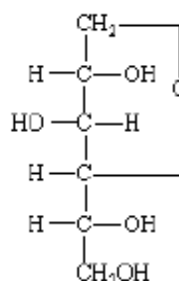
1,4-Sorbitan
