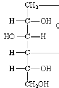
1,4-Sorbitan
